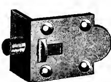
(321) Figs. 4363-4364. DECK-SASH PIVOTS.
